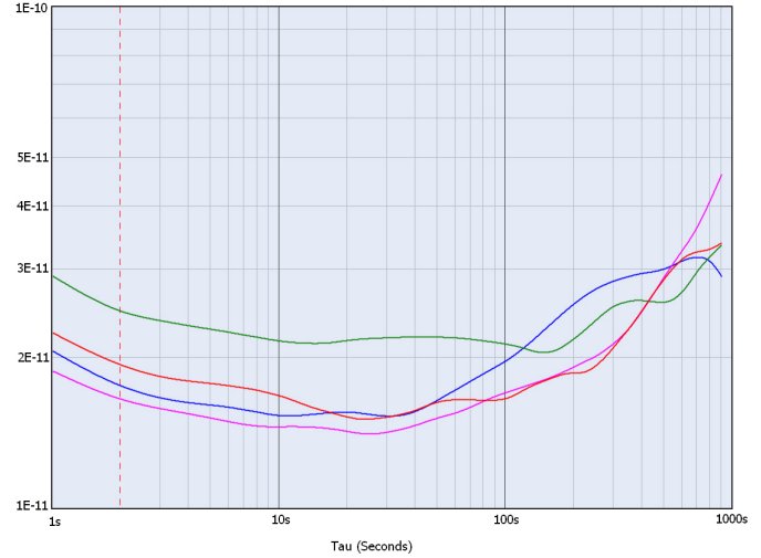
Allan Deviation DOCS012F-024.576M
