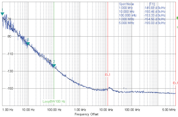
Typical Phase Noise for DOCS012F-024.57M
