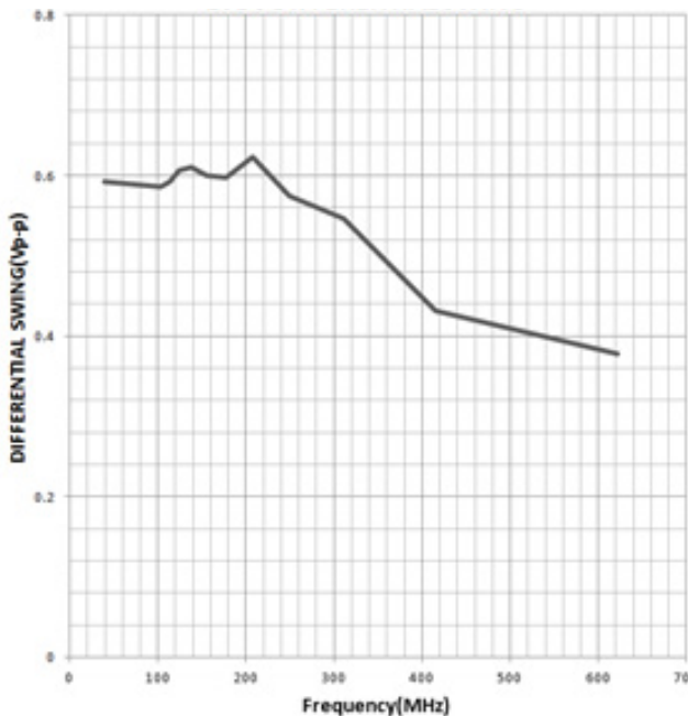
LVDS Differential Swing
