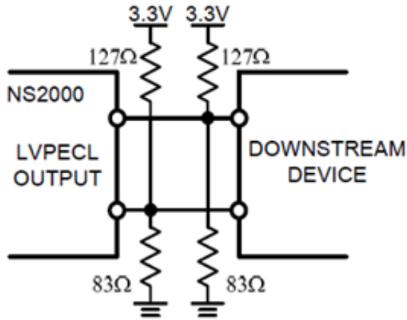
DC-Coupled LVPECL Output Driver
