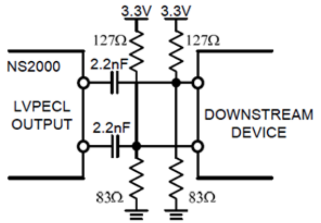
AC-Coupled LVPECL Output Driver
