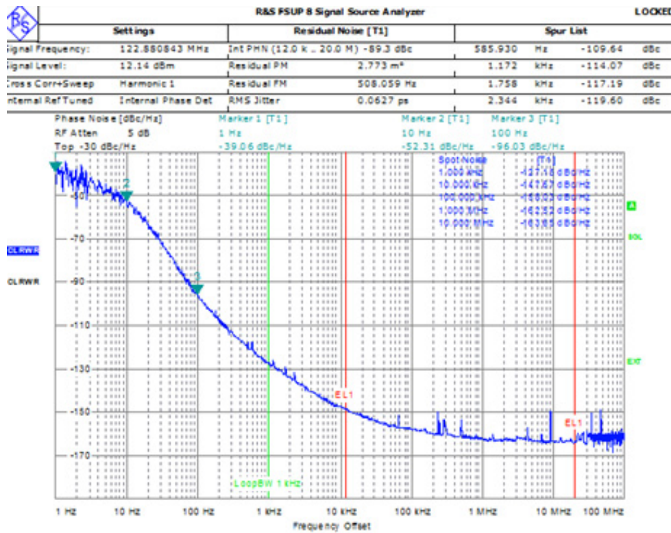
Phase noise generated from PLL1(y): 122.88MHz 63fs (12kHz-20MHz) (using Connor Winfield model V773T-122.88MHz LVC MOS 5x3.2mm VCXO)
