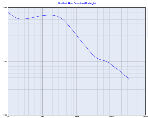
EH320-TFC-CC (in lock mode) Modified Allan Deviation Graph
